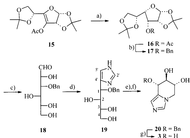
Scheme 3. Conditions and reagents: a) \text{H}_2 , \text{Rh}/\text{Al}_2\text{O}_3 , \text{AcOEt} , 50 bar; b) 1. \text{NaOMe} , \text{Bu}_4\text{NI} , THF, 0^\circ\text{C} ; 2. \text{BnBr} , 50^\circ\text{C} ; c) Dowex, \text{EtOH}/\text{H}_2\text{O} (1:1), 75^\circ\text{C} ; d) \text{H}_2\text{NCH}=\text{NH}/\text{AcOH} , \text{NH}_3 liq., 80^\circ\text{C} , 45 bar; e) \text{TsCl} , pyridine, -10^\circ\text{C} ; f) \text{NaOH} (1 M), acetone, 60^\circ\text{C} , 14 h; g) \text{H}_2 , \text{Pd}(\text{OH})_2 , \text{AcOH}
