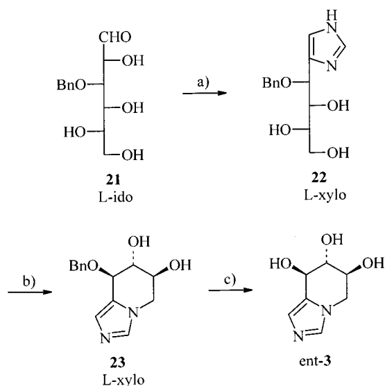
Scheme 4. Conditions and reagents: a) \text{H}_2\text{NCH}=\text{NH}/\text{AcOH} , \text{NH}_3 liq., 90^\circ\text{C} , 40 bar; b) \text{Ph}_3\text{P} , \text{CBr}_4 , DMF, \text{NEt}_3 , 0^\circ\text{C} ; c) \text{H}_2 , \text{Pd}(\text{OH})_2/\text{C} , \text{AcOH}
