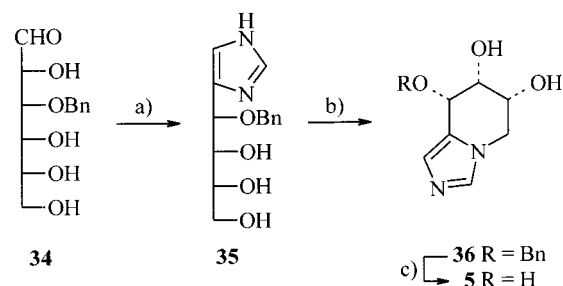
Scheme 7. Conditions and reagents: a) HN=CHNH 2 /AcOH, NH 3 liq., 80 °C, 40 bar; b) Ph 3 P, CBr 4 , NEt 3 , DMF, 40 °C; c) H 2 , Pd(OH) 2 /C, AcOH
