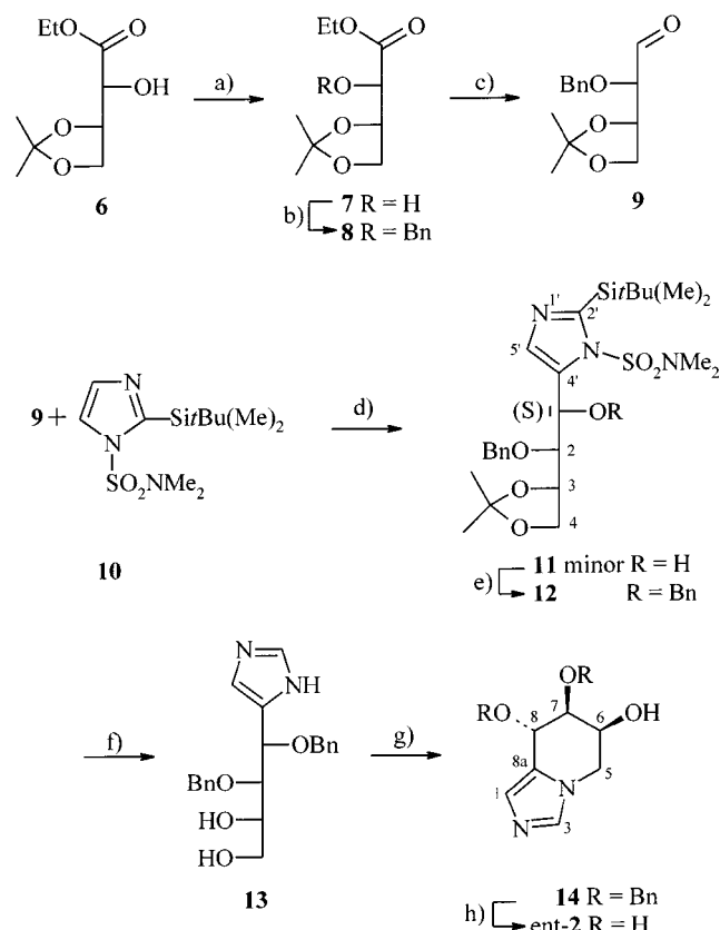
Scheme 2. Reagents and conditions: a) 1. Tf 2 O, pyridine, CH 2 Cl 2 , 0 °C; 2. Bu 4 NNO 2 , CH 2 Cl 2 , 40 °C; b) BnBr, Ag 2 O, KI (cat.), MS (4 Å), toluene, reflux; c) DIBAH, toluene, -78 °C; d) 10 in THF, n BuLi, -78 °C; 2 + 9 in THF at -65 °C to room temp.; e) BnBr, NaH, NBu 4 I, THF; f) 6 N HCl, 45 °C; g) 1. TsCl (2.3 equiv.), NEt 3 , DMAP, CH 2 Cl 2 ; 2. NaOH (1 M), acetone; h) H 2 , Pd(OH) 2 /C, MeOH
